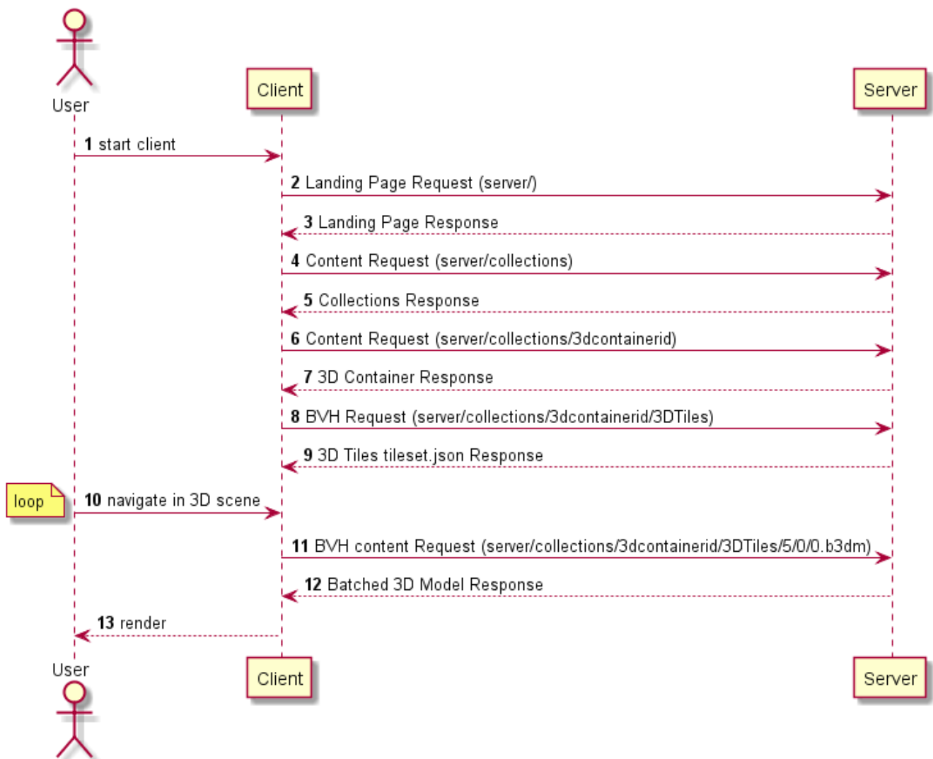
Figure 9. API Sequence Diagram
