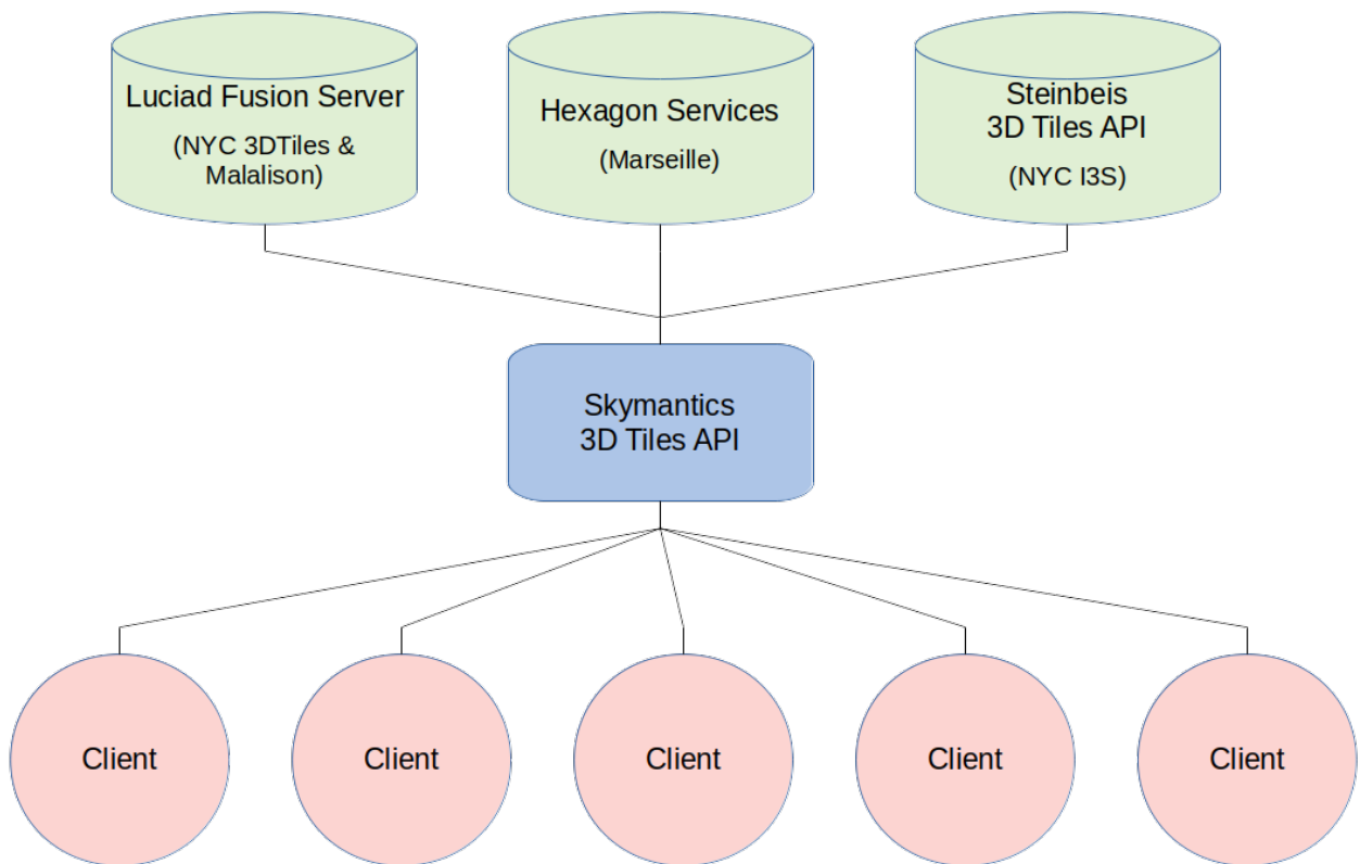
Figure 55. Service Architecture
